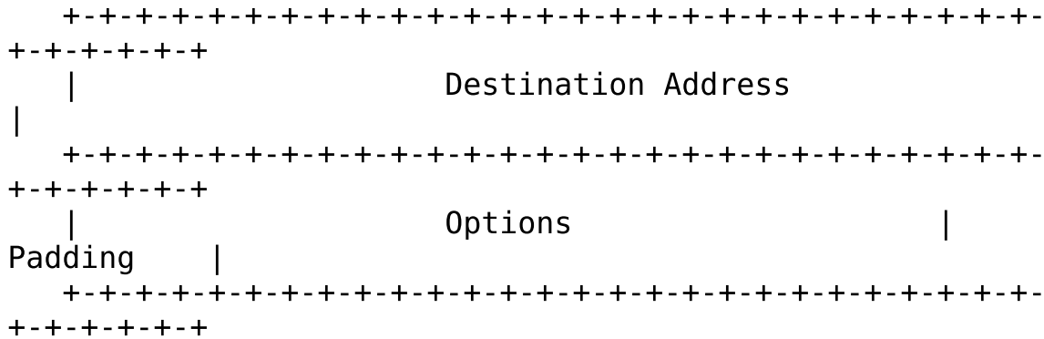
Example Internet Datagram Header
