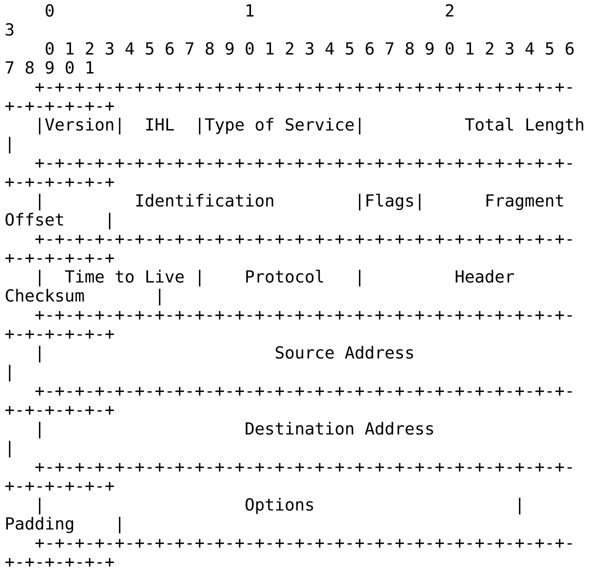
Example Internet Datagram Header
